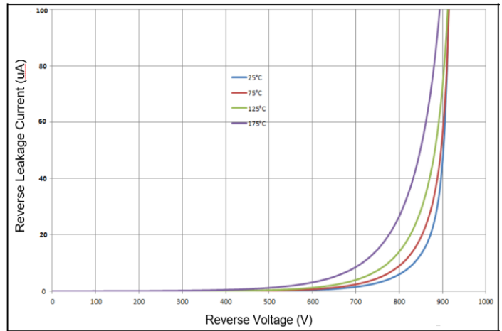
Fig. 2 Reverse Characteristics
