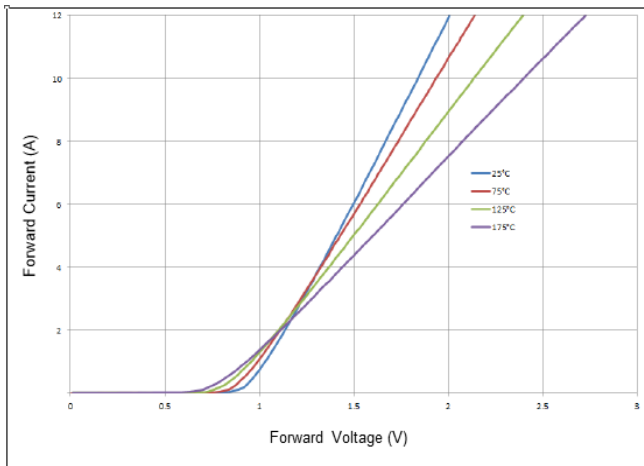
Fig. 1 Forward Characteristics
